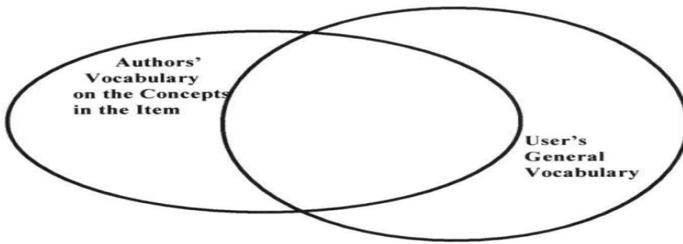
Figure 1.3 Vocabulary Domains
