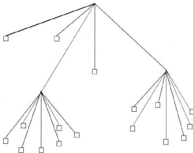
Figure 8.4 Cone Tree
