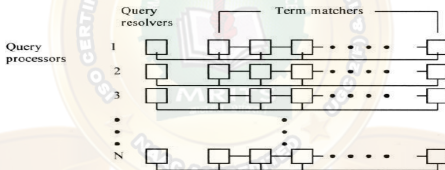
Figure 9.10 GESCAN Text Array Processor
