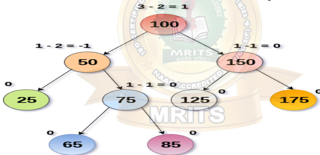
AVL Tree
